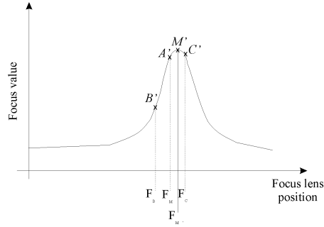
Fig. 7. Autofocus algorithm
